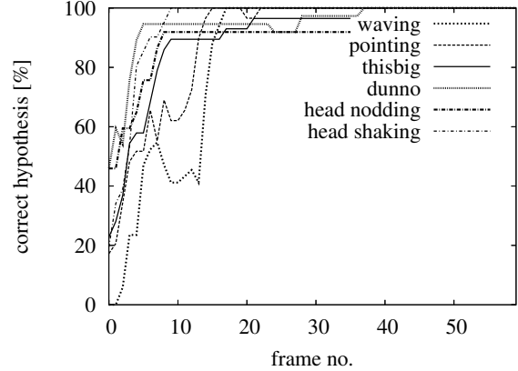
Fig. 5. Number of frames after which the most likely hypothesis is the correct gesture.
