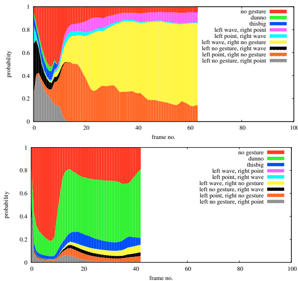
Fig. 6. Evolution of the probabilities of the gestures over time for waving with the left hand (top image) and Dunno (bottom image).
