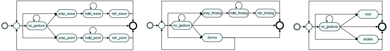
Fig. 4. Composed HMMs consisting of the individual phase-HMMs. The first two for one- and two-handed gestures, and the right one for head gestures. The start and end states of the HMMs as well as the branching points are non-emitting.
