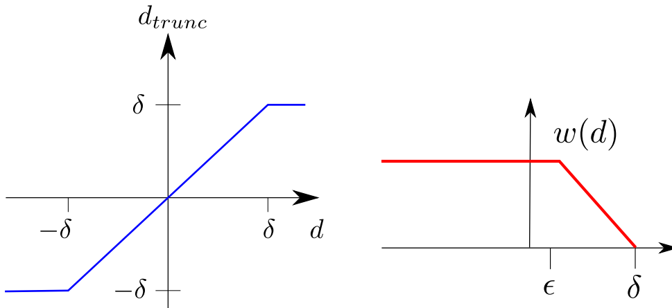
(a) truncated signed distance function (b) weights as a function of the signed distance
