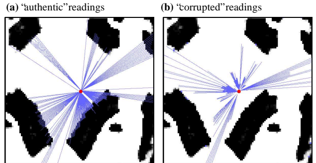
Figure 5: Filtering out corrupted sensor data in dynamic environments: (a) Authentic readings only; (b) readings corrupted by people. Only authentic readings are used for localization. Corrupted readings are employed to find people, e.g., when determining the robot’s mood.
